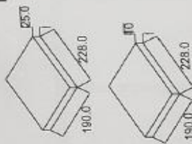
MS plates (Stabilized mud blocks)
