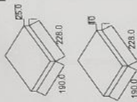
MS plates (Stabilized mud blocks)
